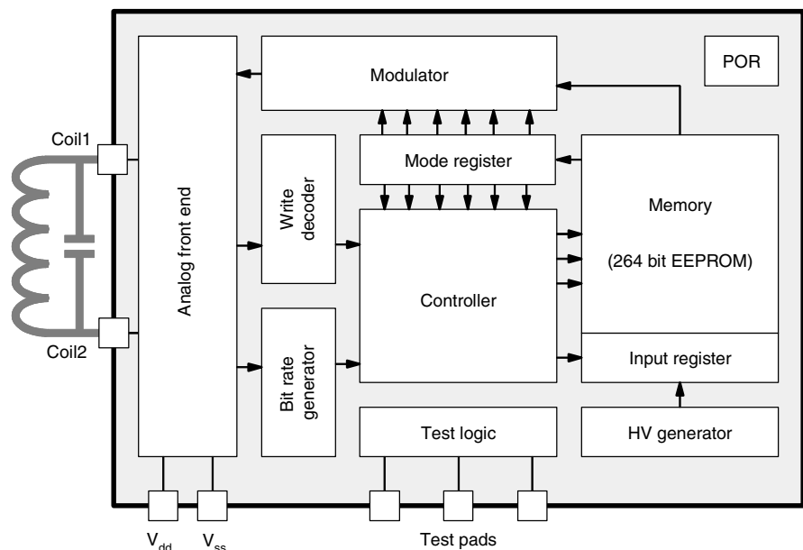
Figure 2. Block Diagram of the e5551
