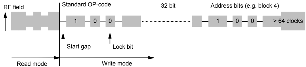
Figure 8. Write Protocol
